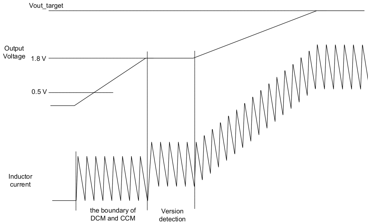
Figure 7-3. Soft-Start Timing
