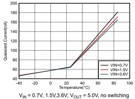
Figure 6-8. Quiescent Current into VOUT vs Temperature
