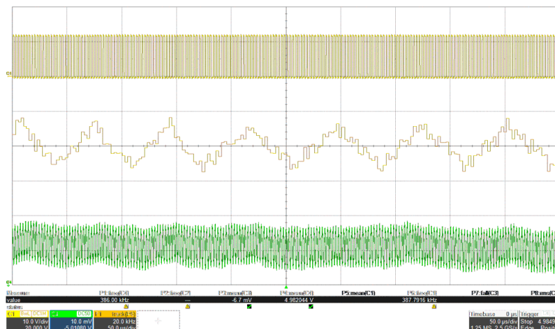
Figure 8-4. Output Ripple with Ripple Cancellation Showing V_{\text{sw}} (Top), F_{\text{sw}} (Middle), V_{\text{OUT}} (Bottom)
