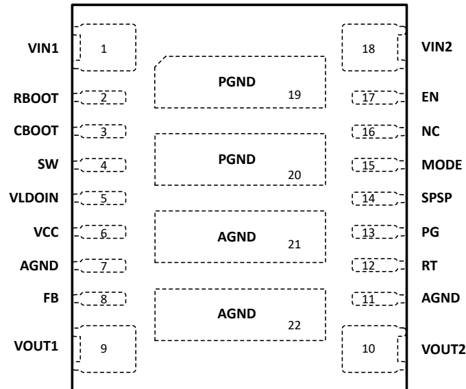
Figure 6-1. 22-Pin B3QFN RDF Package (Top View)
