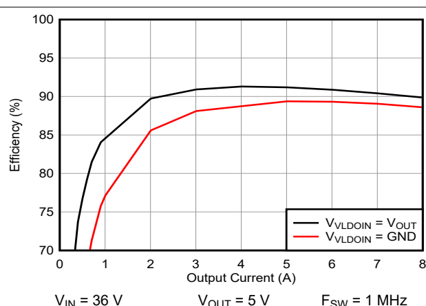
Figure 8-7. Efficiency Increase with External Bias
