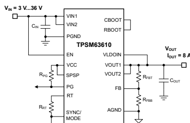
Typical Schematic
