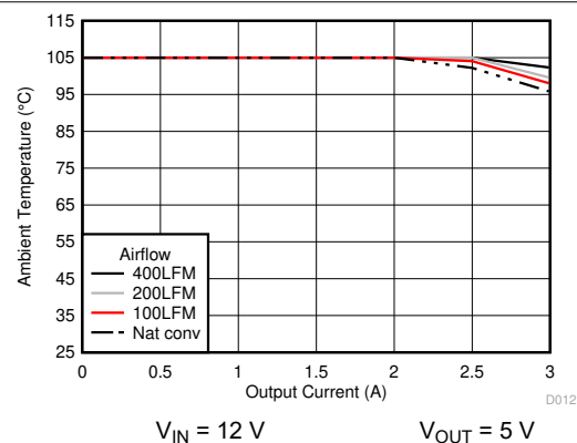
Figure 6-12. Safe Operating Area
