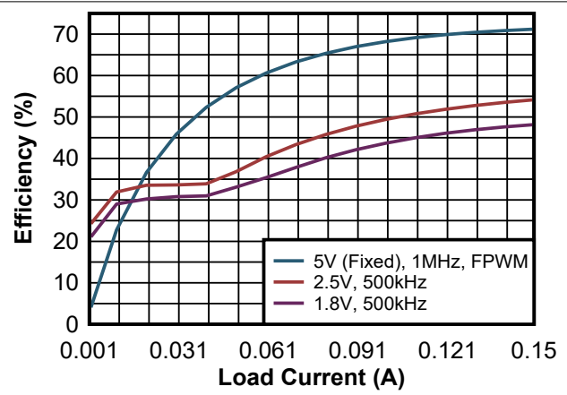
Figure 8-10. 48VIN Efficiency
