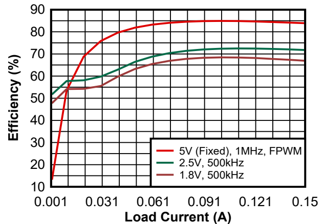
Figure 8-6. 12VIN Efficiency
