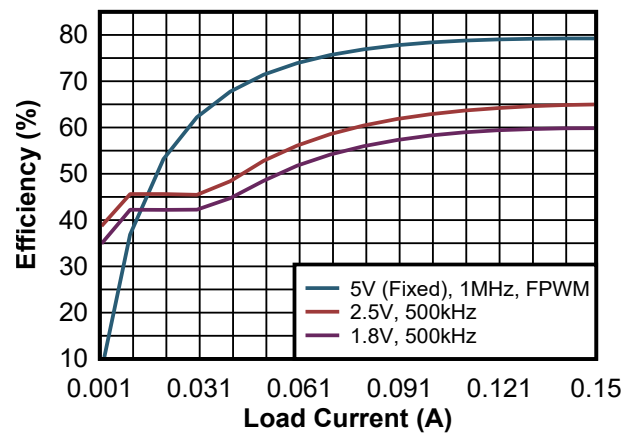
Figure 8-8. 24VIN Efficiency
