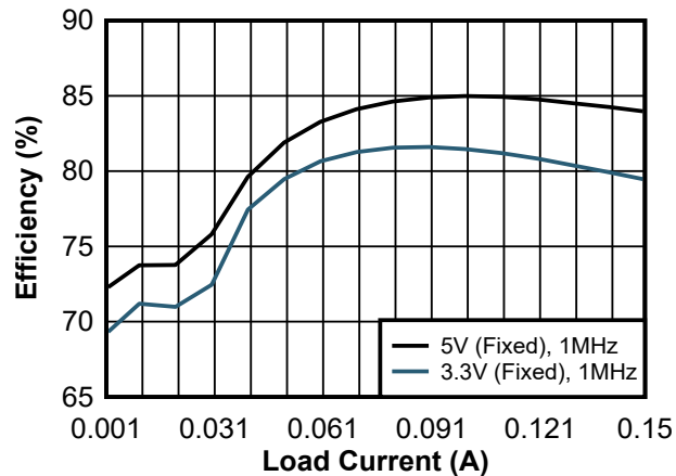
Figure 8-5. 12VIN Efficiency
