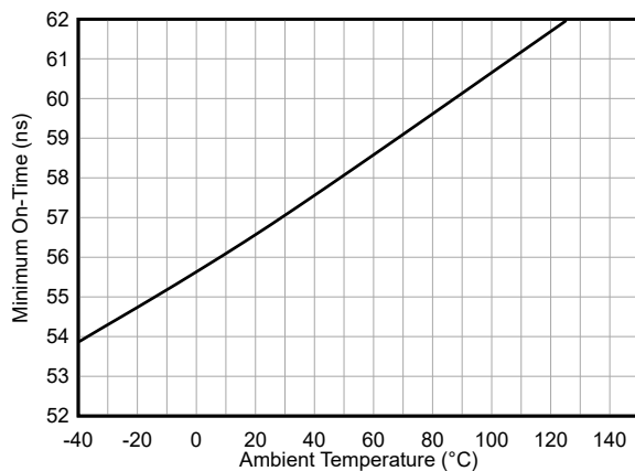
Figure 6-5. Minimum On-Time vs Temperature
