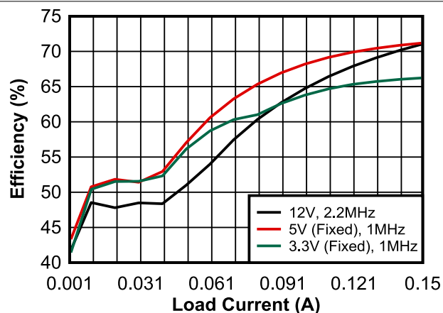
Figure 8-9. 48VIN Efficiency
