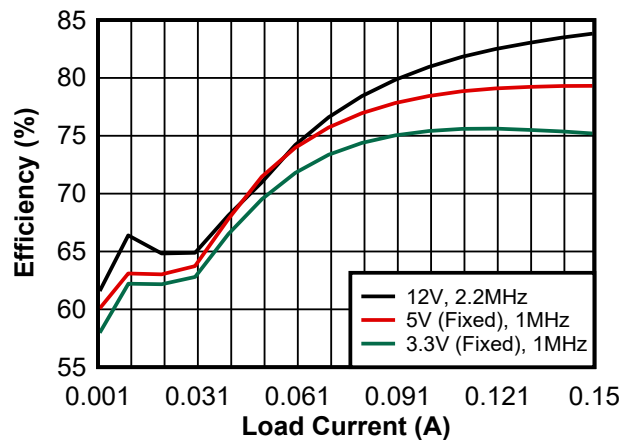
Figure 8-7. 24VIN Efficiency
