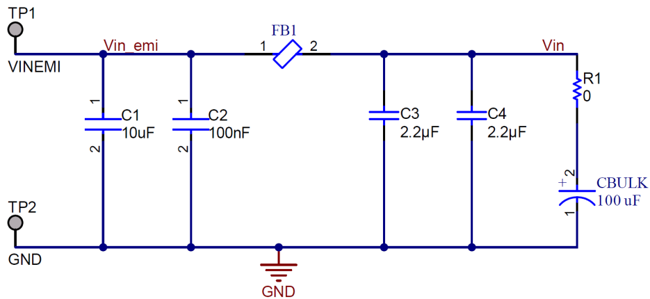
Figure 8-18. Typical Input EMI Filter
