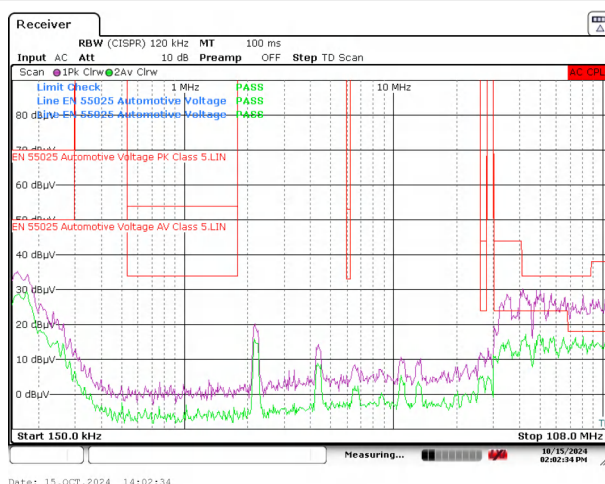
Figure 8-6. CISPR 25, CE Scan 150kHz – 108MHz, (Purple Peak, Green AVG), 12VIN, 3.3VOUT, 2.2MHz, 2A Load Current
