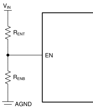
Figure 7-6. Setup for External UVLO Application
