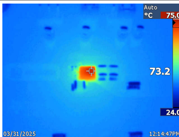
Figure 8-8. Thermal Capture, 36VIN, 3.3VOUT, 2.2MHz, 2A Load Current
