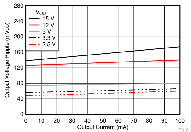
Figure 6-14. Output Voltage Ripple C_{OUT} = 47 \mu\text{F} , 16-V, ceramic
