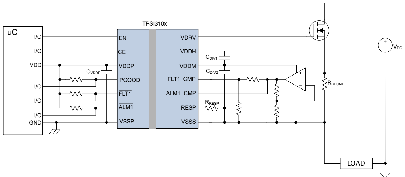
Figure 9-2. TPSI310x-Q1 overcurrent protection with current sense amplifier, fault and alarm indicators
