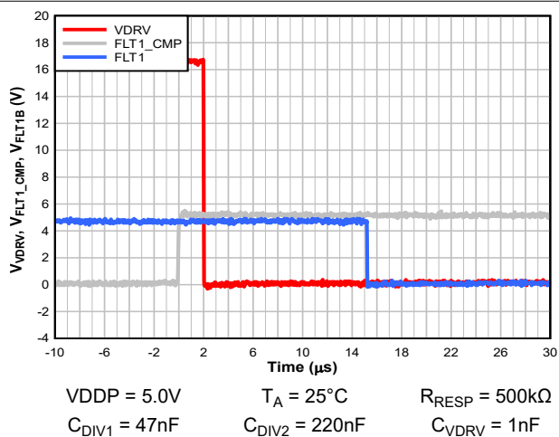
Figure 6-12. t PD_CMP_VDRV_DIS , t FLT_LATENCY
