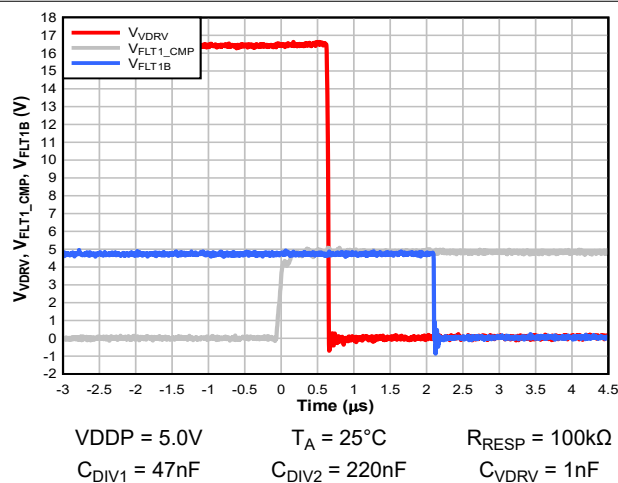
Figure 6-11. t PD_CMP_VDRV_DIS , t FLT_LATENCY
