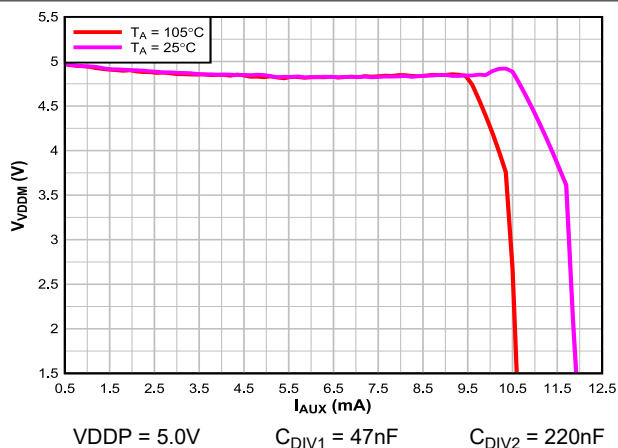
Figure 6-10. V_VDDM versus I_AUX
