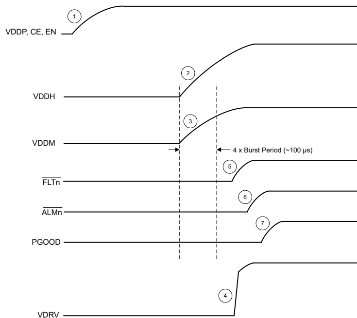
Figure 8-12. TPSI310x Typical Start-up (CE = EN = VDDP, \overline{\text{FLTn\_CMP}} = 0 , \overline{\text{ALMn\_CMP}} = 0 )
