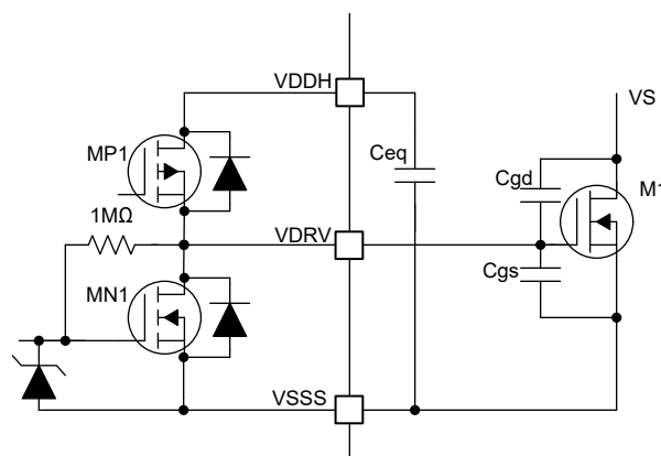
Figure 8-9. Keep-Off Circuitry
