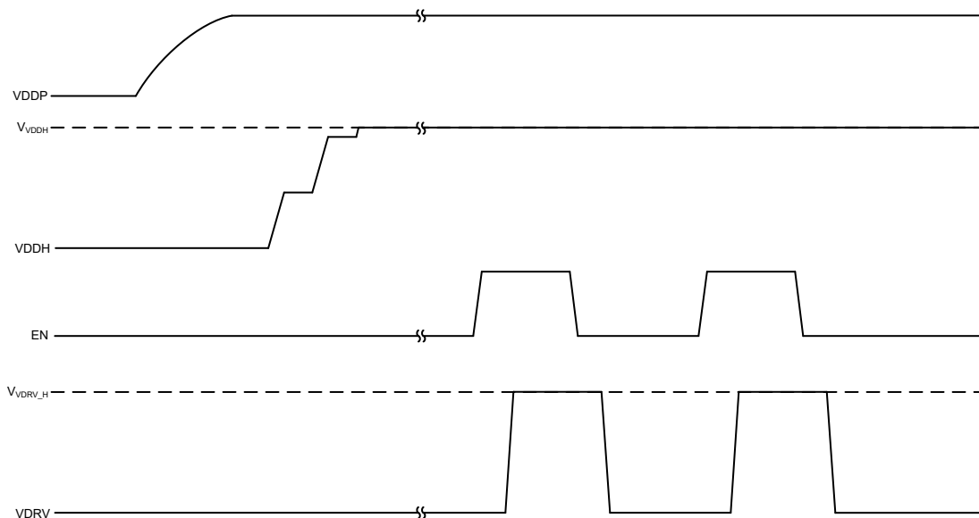
Figure 8-2. Three-Wire Mode with TPSI3052-Q1 (Standard Enable)
