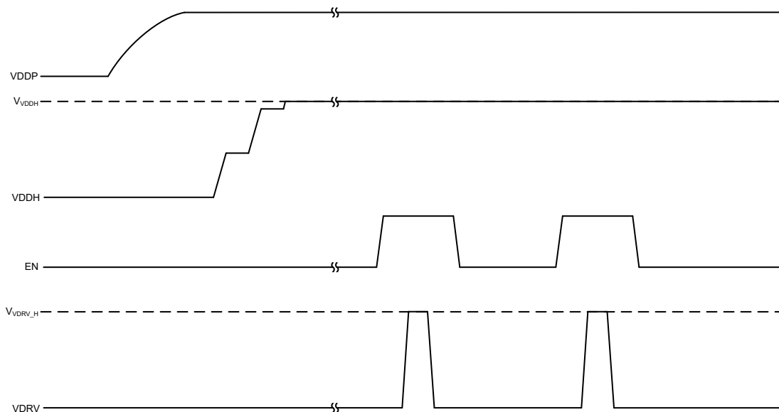
Figure 8-3. Three-Wire Mode with TPSI3052S-Q1 (One-shot Enable)
