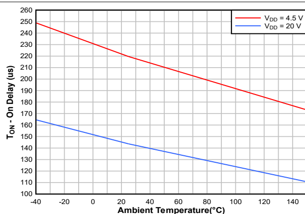
Figure 6-7. Input to Output ON Delay ( V_{IN} = 1000\text{V} )
