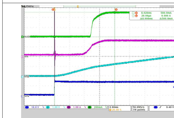
Ch1: Input voltage; Ch2: Soft-start (SS) voltage; Ch3: Input current; Ch4: LED current; Time: 2 ms/div
