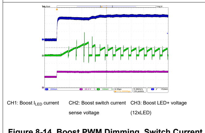
Figure 8-14. Boost PWM Dimming, Switch Current
