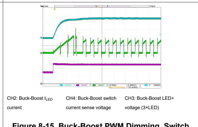
Figure 8-15. Buck-Boost PWM Dimming, Switch Current
