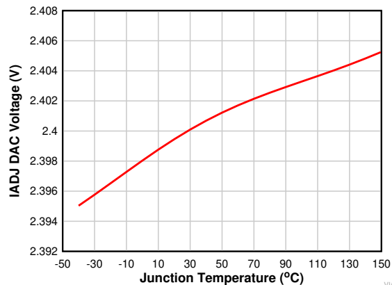
Figure 6-17. VIADJ Voltage vs Junction Temperature
