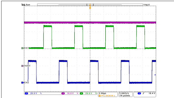
CH1: Phase-1 V_{SW} CH2: Phase-2 V_{SW} CH3: CV Boost V_{OUT} voltage voltage
