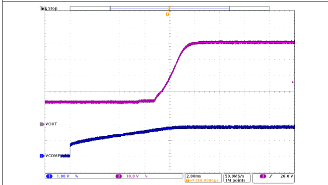
CH1: V_{COMP1} pin CH3: CV Boost V_{OUT} Figure 8-27. Start-up, SOFTSTART = 0111
