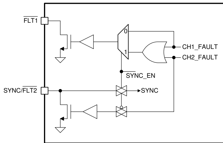
Figure 7-14. Fault PINs
