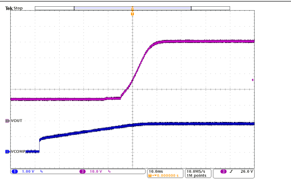
CH1: V_{COMP1} pin CH3: CV Boost V_{OUT} Figure 8-28. Start-up, SOFTSTART = 1111
