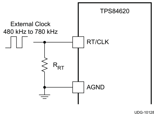
Figure 36. CLK/RT Configuration
