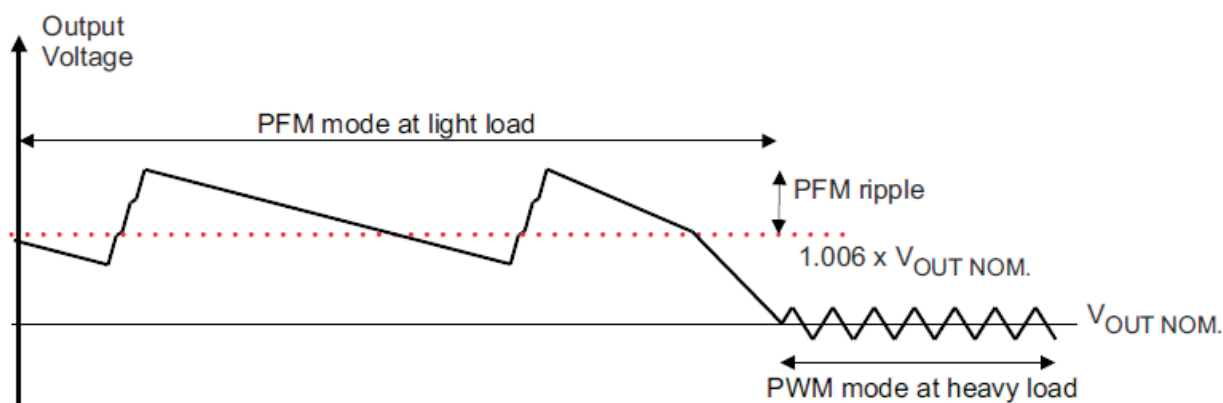
Figure 12. Power-Save Example
