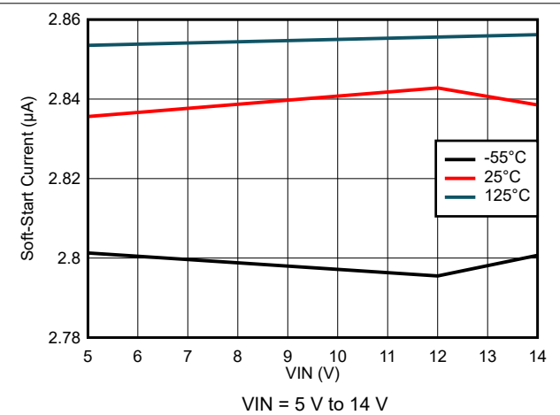
Figure 7-10. Soft-Start Current Variation
