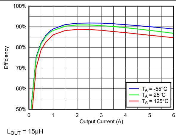
Figure 7-12. Efficiency vs Load Across Temperature at 100kHz, V_{IN} = 12V , V_{OUT} = 1.8V
