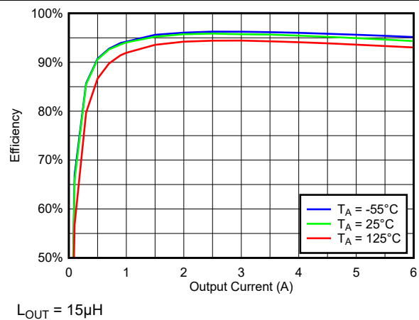
Figure 7-10. Efficiency vs Load Across Temperature at 100kHz, V_{IN} = 12V , V_{OUT} = 5V
