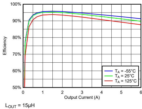
Figure 7-7. Efficiency vs Load Across Temperature at 100kHz, V_{IN} = 5V , V_{OUT} = 2.5V
