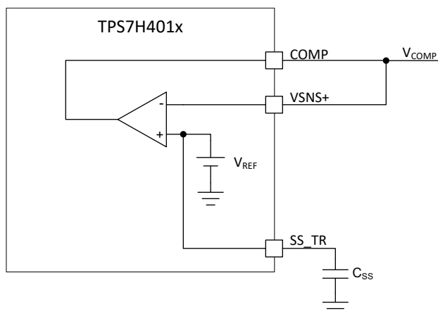
Figure 8-1. Reference Voltage Measurement
