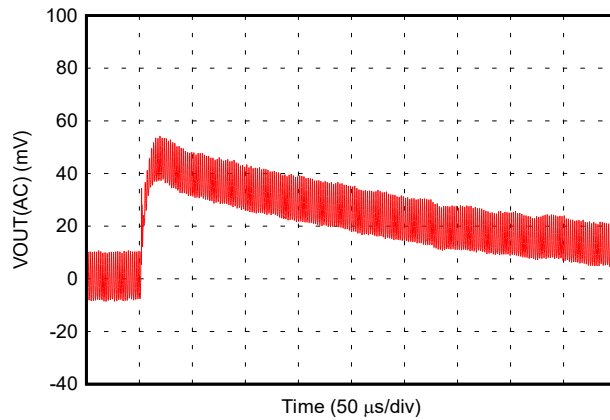
Figure 7-55. Falling Load Step: 5.5A to 0A at 226A/ \mu s
