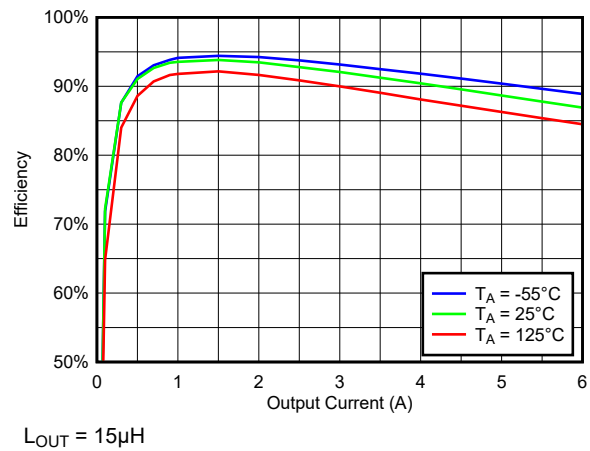
Figure 7-8. Efficiency vs Load Across Temperature at 100kHz, V_{IN} = 5V , V_{OUT} = 1.8V
