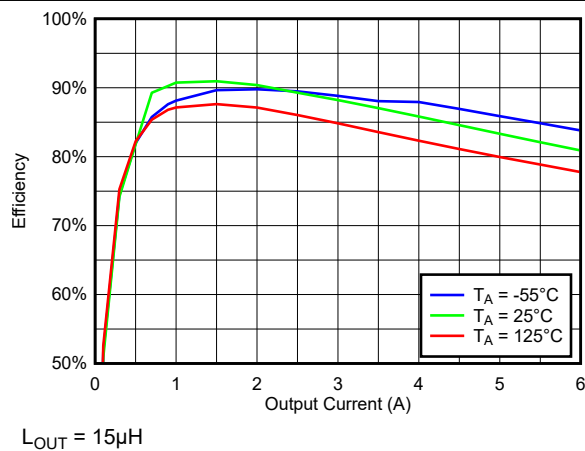
Figure 7-9. Efficiency vs Load Across Temperature at 100kHz, V_{IN} = 5V , V_{OUT} = 1.1V
