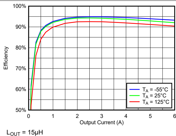
Figure 7-11. Efficiency vs Load Across Temperature at 100kHz, V_{IN} = 12V , V_{OUT} = 3.3V
