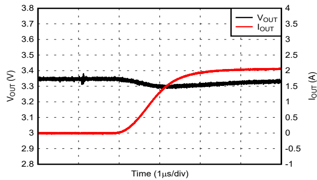
Figure 6-23. Load Step: 0A to 2A with V_{IN} = 5V
