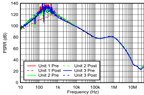
Figure 9-6. PSRR with I_{OUT} = 100 mA
