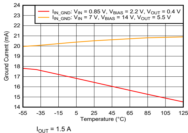
Figure 6-34. Ground Current vs Temperature
