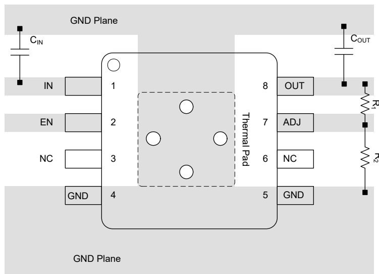
Figure 7-10. Example Layout for TPS7E82-Q1 DGN Package
