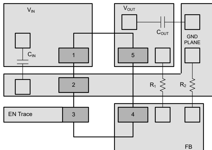
Figure 7-7. Example Layout for TPS7E82-Q1 (With EN) DBV Package
