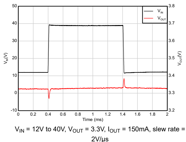
Figure 5-32. Line Transient
