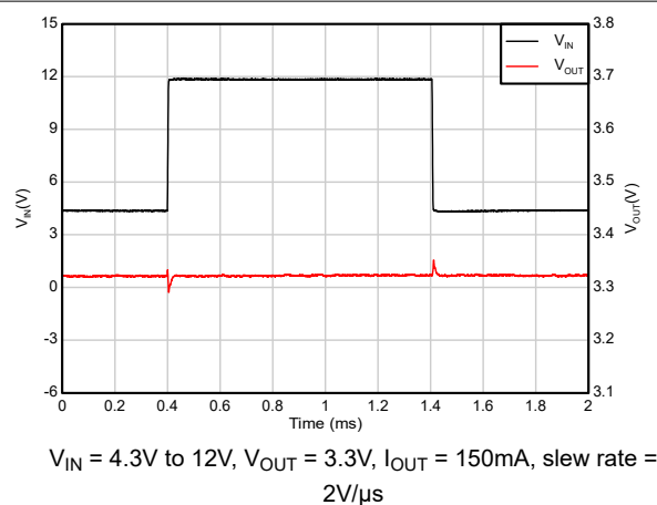
Figure 5-30. Line Transient
