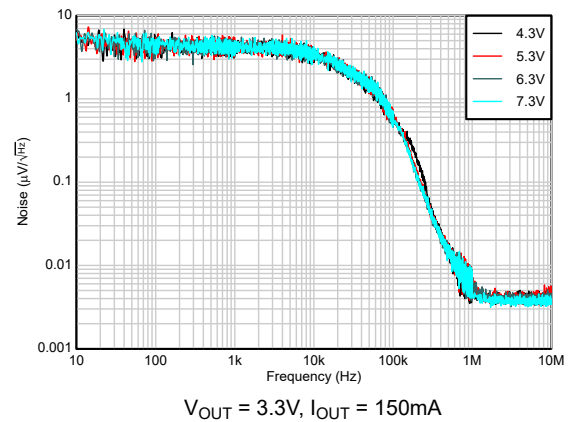
Figure 5-24. Output Noise vs Frequency, Input Voltage
