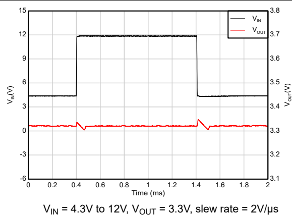
Figure 5-29. Line Transient
