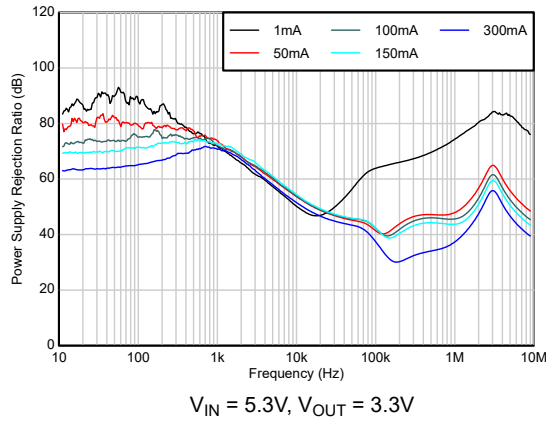
Figure 5-21. Ripple Rejection vs Frequency, Output Current
