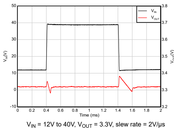
Figure 5-31. Line Transient
