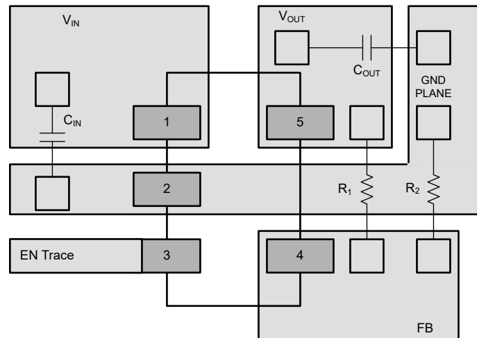
Figure 7-6. Example Layout for TPS7E82 DBV Package
