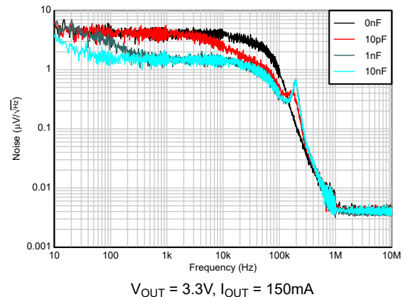
Figure 5-26. Output Noise vs Frequency, C_{FF}
