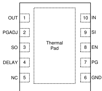
Figure 5-1. DRC Package, 10-Pin VSON, Top View
