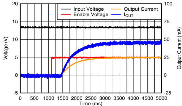
Figure 8-13. Power-Up Waveform
