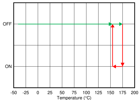
Figure 6-37. Thermal Shutdown
