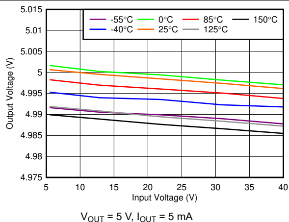
Figure 6-3. Line Regulation vs V_{IN}
