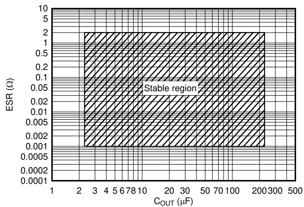
Figure 6-38. Stability ESR vs C_{OUT}
