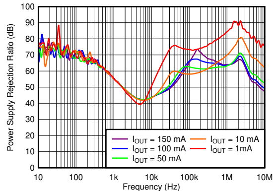
Figure 8-14. PSRR
