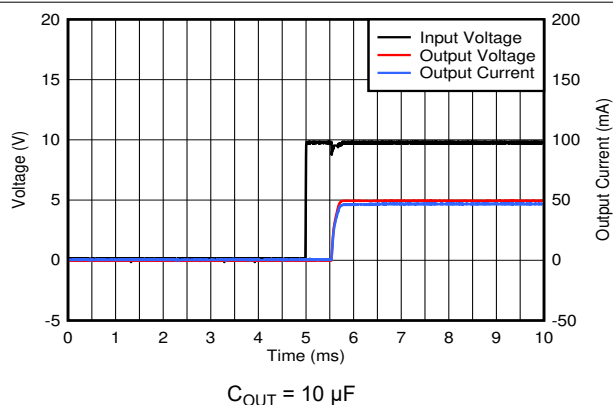
Figure 6-34. Startup Plot
