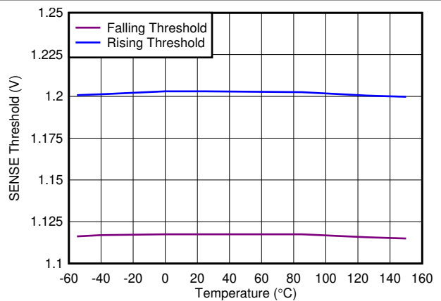
Figure 6-28. Undervoltage Lockout (UVLO) Threshold vs Temperature
