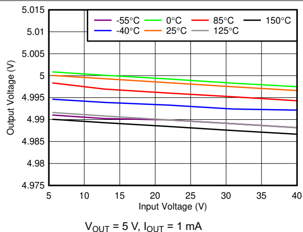
Figure 6-4. Line Regulation vs V_{IN}
