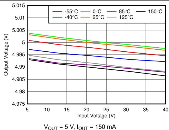
Figure 6-2. Line Regulation vs V_{IN}
