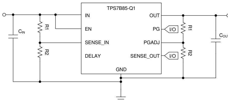
Figure 8-6. Monitoring the Device Input Voltage
