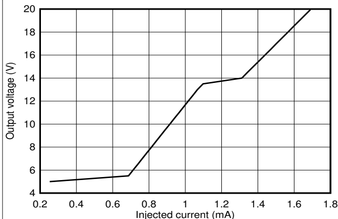
Figure 6-34. Startup Plot
