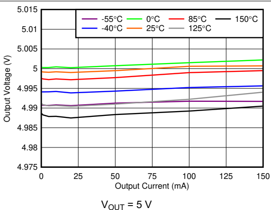
Figure 6-5. Load Regulation vs I_{OUT}
