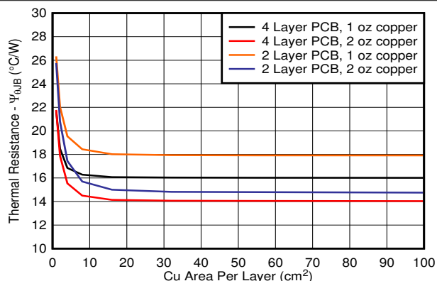
Figure 8-3. \psi_{JB} vs Copper Area 2s2p DRC Package
