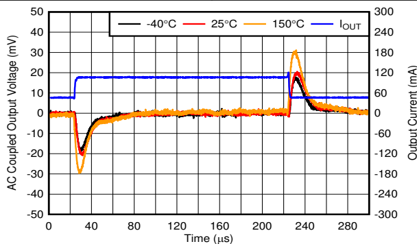
Figure 8-15. Transient Response
