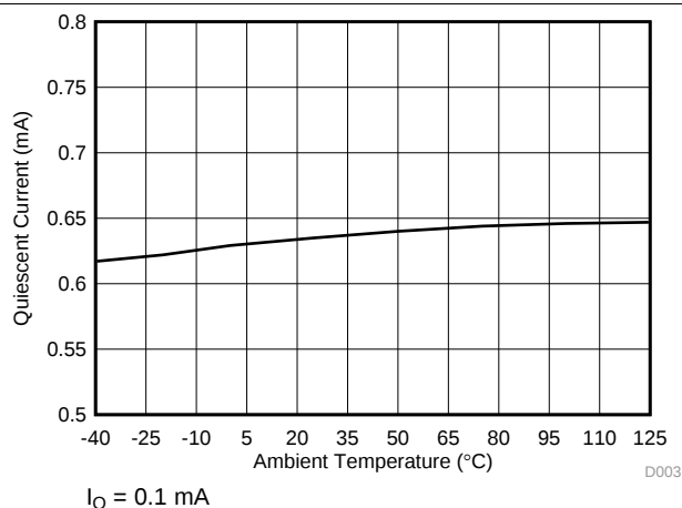
Figure 4. Quiescent Current vs Ambient Temperature (TPS7B7702-Q1)
