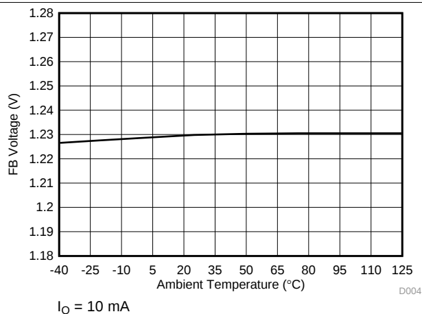
Figure 6. FB Voltage vs Ambient Temperature
