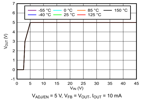
Figure 5-4. Output Voltage vs Input Voltage
