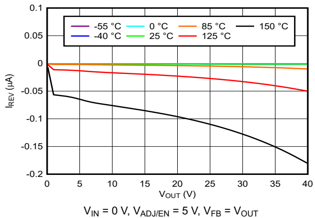
Figure 5-16. Reverse Current vs Output Voltage
