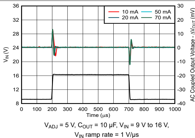
Figure 6-18. Line Transient
