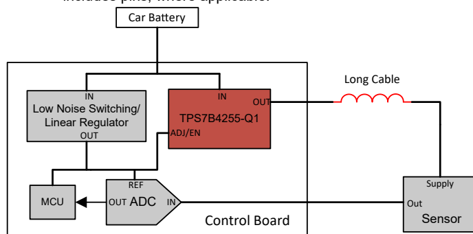
Typical Application
