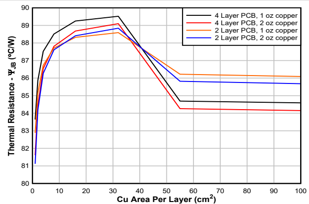
Figure 8-7. \psi_{JB} vs Copper Area (DBV Package)
