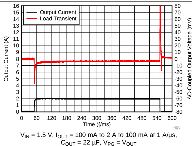
Figure 29. Load Transient Response ( V_{OUT} = 1.2\text{ V} )
