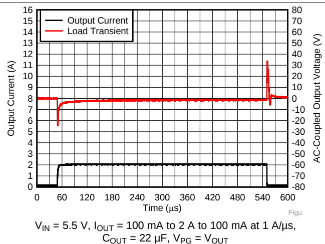
Figure 30. Load Transient Response ( V_{OUT} = 5.0\text{ V} )
