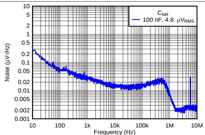
Figure 41. Output Noise vs Frequency
