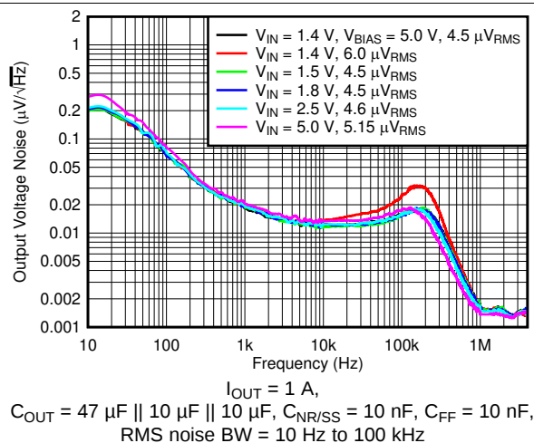
Figure 11. Output Noise vs Frequency and Input Voltage
