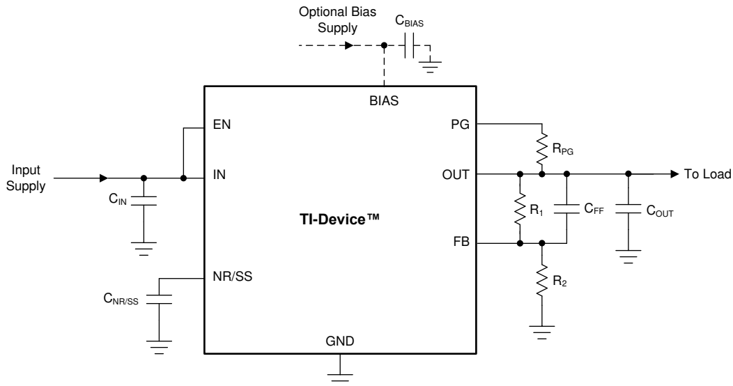
Figure 44. Typical Circuit
