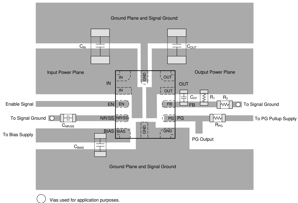
Figure 55. Example Layout
