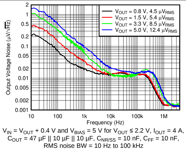
Figure 10. Output Noise vs Frequency and V_{OUT}
