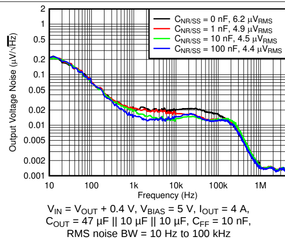
Figure 12. Output Noise vs Frequency and C_{NR/SS}
