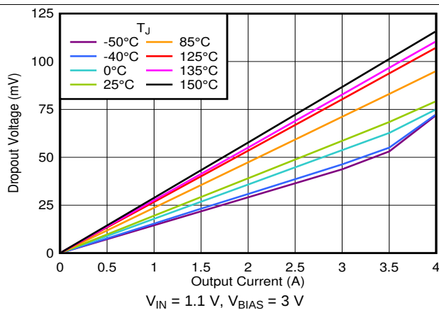
Figure 23. Dropout Voltage vs Output Current With Bias
