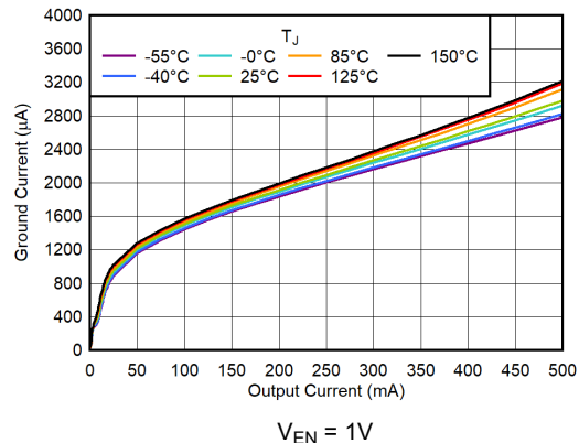
Figure 5-10. I_{GND} vs I_{OUT}
