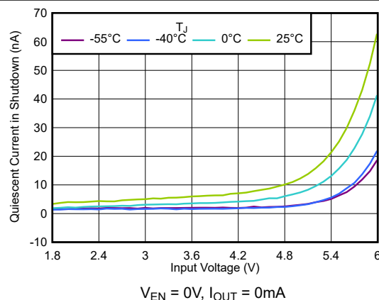
Figure 5-12. Shutdown Current vs V_{IN}
