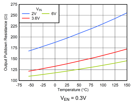
Figure 5-18. Output Pulldown Resistance vs Temperature and V_{IN}
