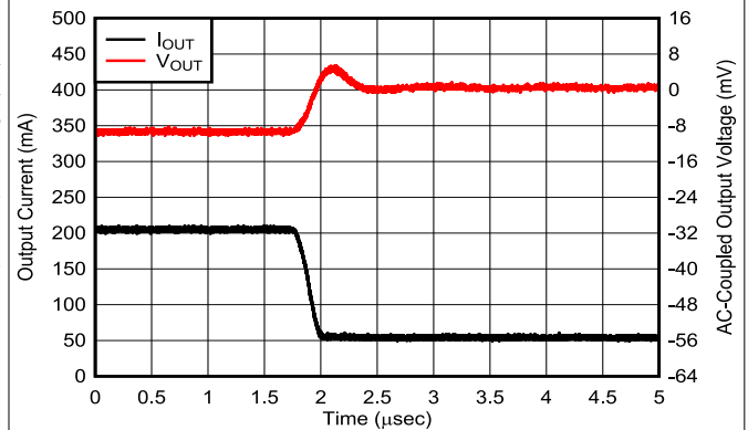
Figure 5-16. Load Transient
