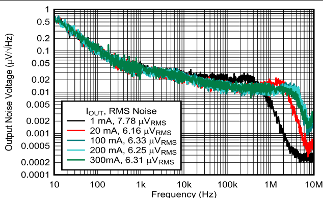
Figure 5-31. Noise vs Frequency and I_{OUT}
