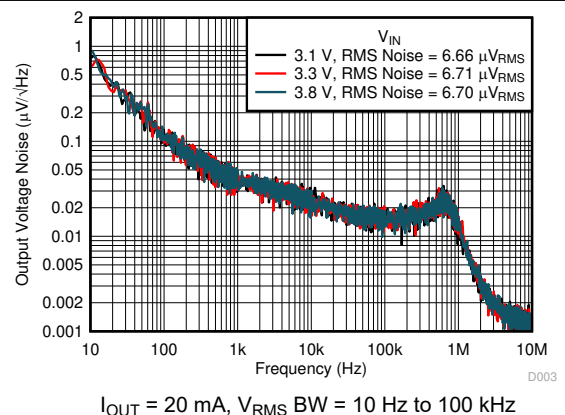
Figure 5-66. Noise vs Frequency and V_{IN}
