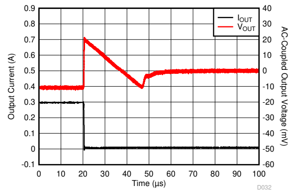
Figure 5-52. Load Transient
