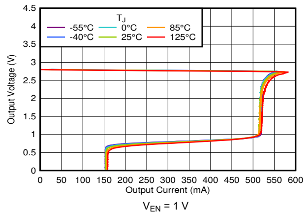
Figure 5-44. Current Limit
