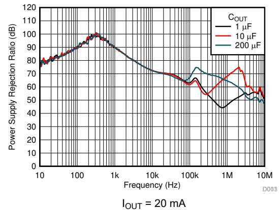
Figure 5-64. PSRR vs Frequency and C_{OUT}
