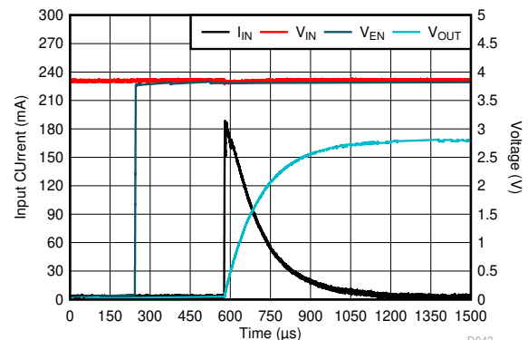
Figure 5-82. Start-Up
