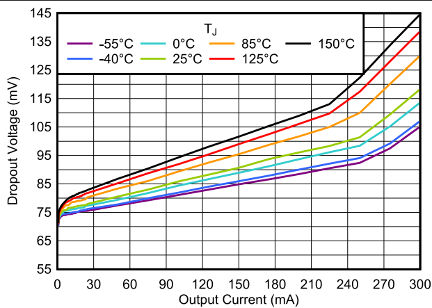
Figure 5-25. Dropout Voltage vs I_{OUT}
