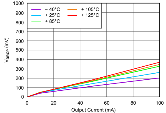
Figure 6-4. Dropout Voltage vs Output Current
