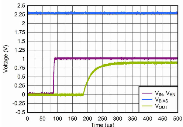
Figure 6-14. Start-Up With V_{\text{BIAS}} Before V_{\text{IN}}
