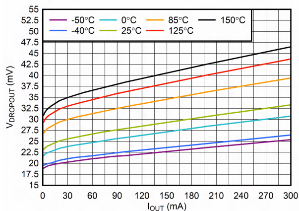
Figure 8-5. V_{\text{IN}} Dropout Voltage vs I_{\text{OUT}}
