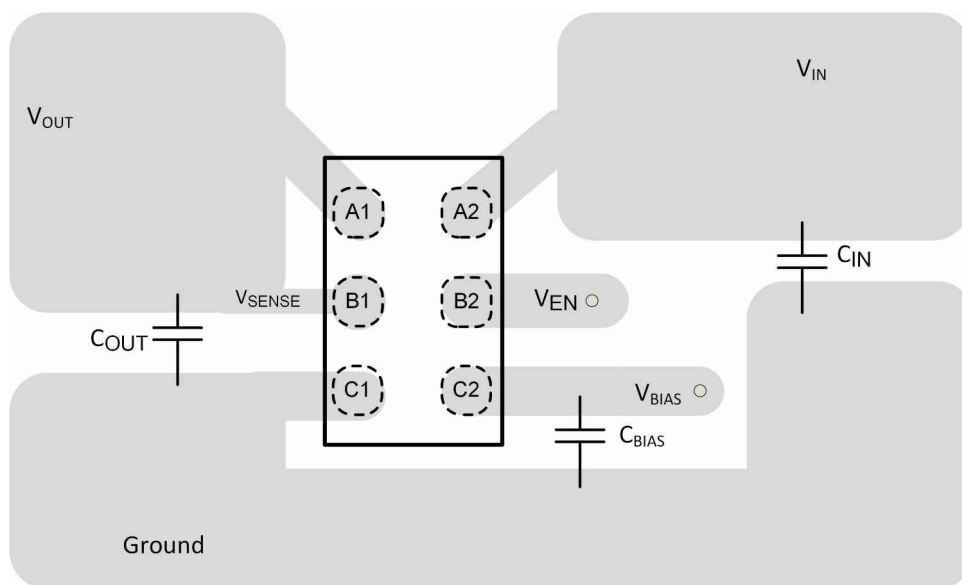
Figure 10-1. Recommended Layout
