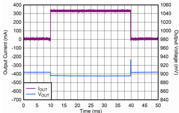
Figure 6-20. Load Transient From 100 \mu\text{A} to 320 mA
