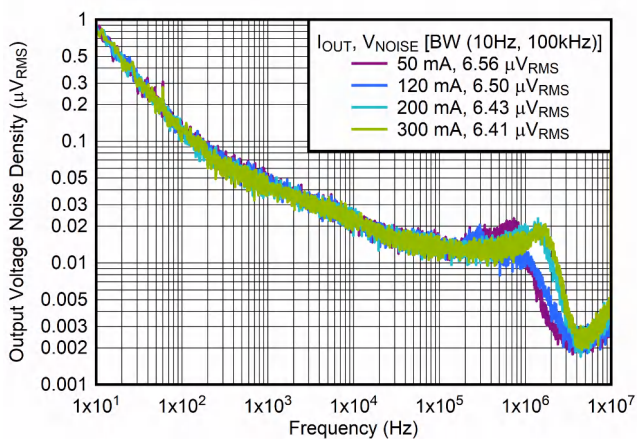
Figure 6-26. Output Noise vs Frequency and I_{\text{OUT}}
