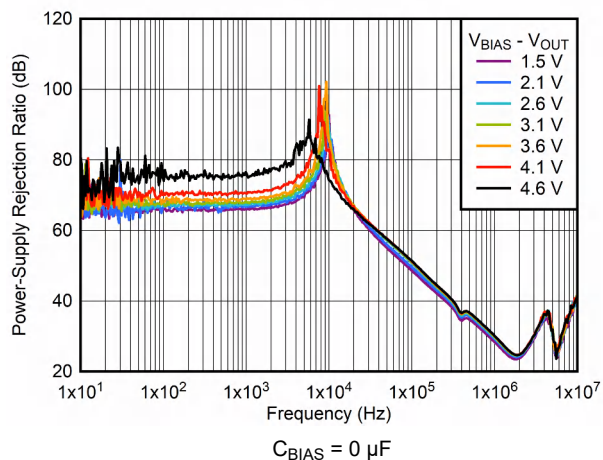
Figure 6-25. V_{\text{BIAS}} PSRR vs Frequency and V_{\text{BIAS}} - V_{\text{OUT}}
