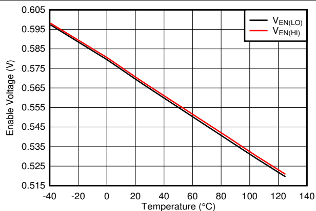
Figure 6-32. Enable High and Low Threshold vs Temperature
