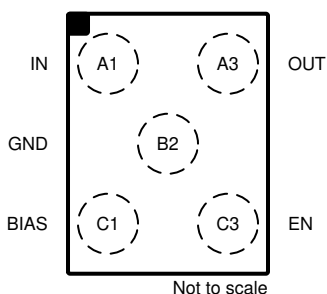
Figure 5-2. YKA Package, 5-Pin DSBGA, Top View
