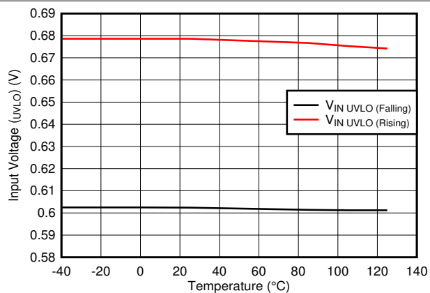
Figure 6-31. V_{UVLO(IN)} Rising and Falling Threshold vs Temperature
