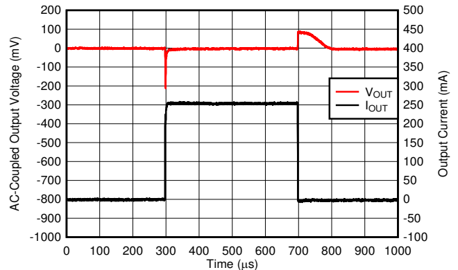
Figure 6-20. I_{OUT} Transient
