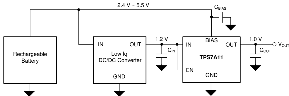
Figure 8-4. High Efficiency Supply From a Rechargeable Battery
