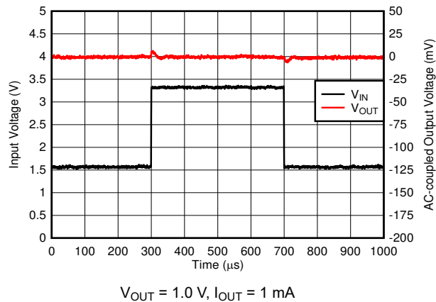
Figure 6-18. V_{IN} Transient
