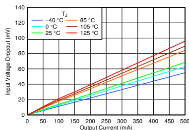
Dropout vs I_{OUT} and Temperature, YKA Package
