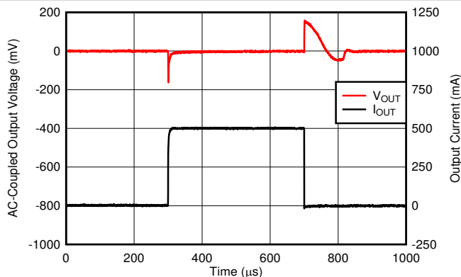
Figure 6-21. I_{OUT} Transient
