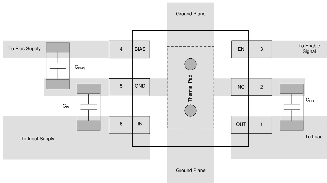
Figure 10-2. Recommended Layout for DRV Package
