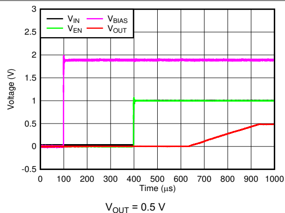
Figure 6-14. Startup With V_{EN} = V_{IN}
