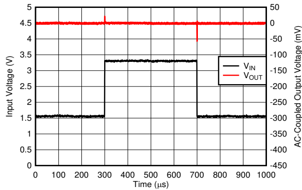
Figure 6-19. V_{IN} Transient
