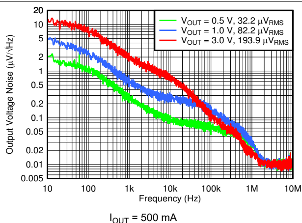
Figure 6-29. Output Noise vs Frequency and V_{OUT}
