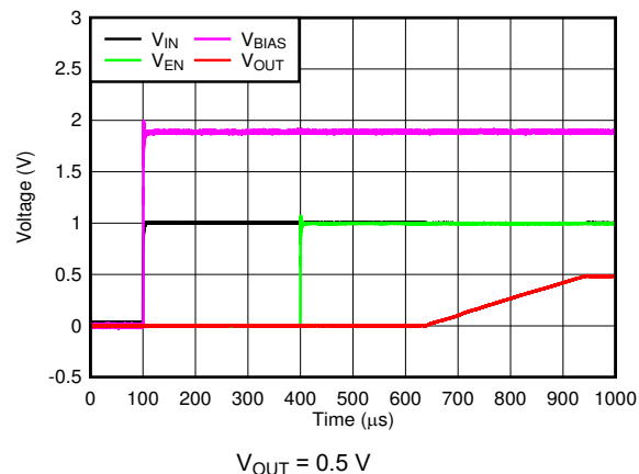
Figure 6-16. Startup With Separated V_{EN}
