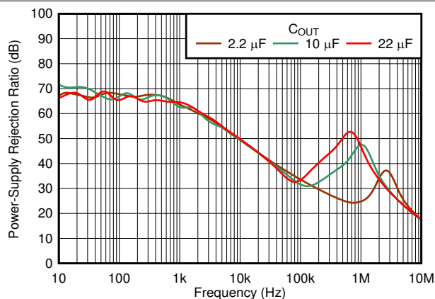
Figure 6-26. V_{IN} PSRR vs Frequency and C_{OUT}
