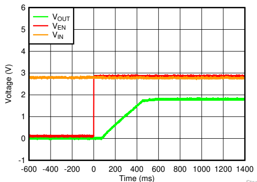
Figure 6-51. Startup With V_{EN} = V_{IN}
