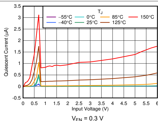
Figure 6-12. I_{SHDN} vs V_{IN}
