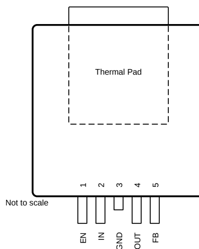
Figure 5-6. KVV Package (Adjustable), 5-Pin TO-252 (Top View)
