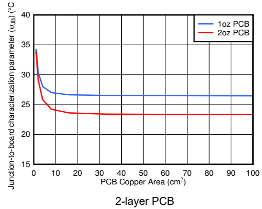
Figure 10-4. Junction-to-Board Characterization Parameter ( \psi_{JB} ) vs PCB Copper Area (DRB Package)
