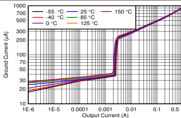
Figure 6-8. I_{GND} vs I_{OUT}
