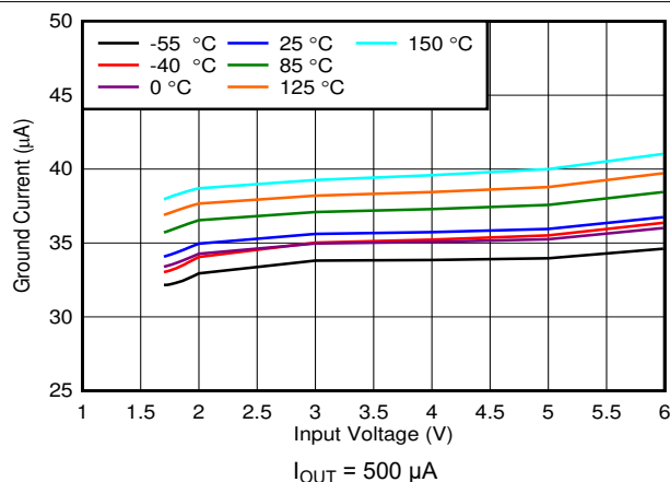
Figure 6-7. I_{GND} vs V_{IN}
