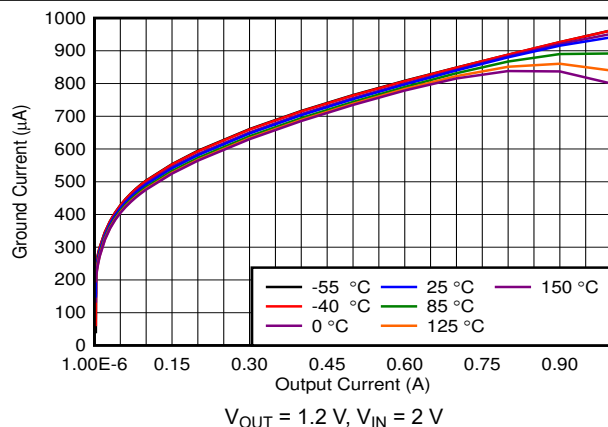
Figure 6-9. I_{GND} vs I_{OUT}
