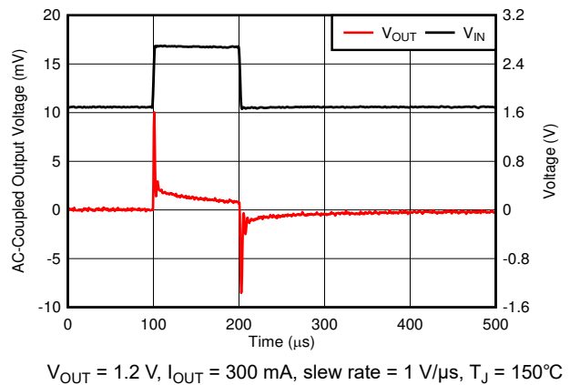
Figure 6-34. Line Transient
