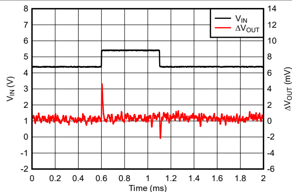
Figure 7-11. TPS76933 Line Transient Response (New Chip)
