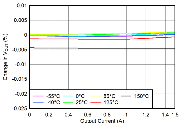
Figure 7-8. Load Regulation
