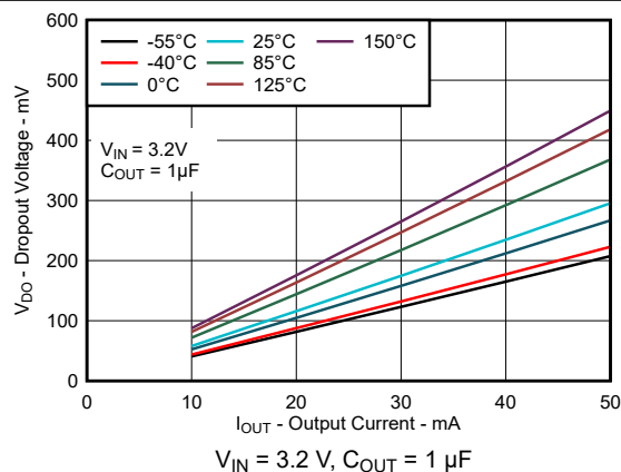
Figure 6-10. Dropout Voltage vs Output Current for New Chip
