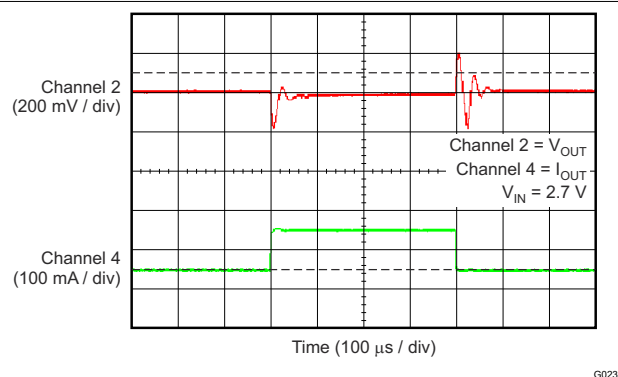
Figure 6-22. TPS70912 Load Transient (1 mA to 150 mA)
