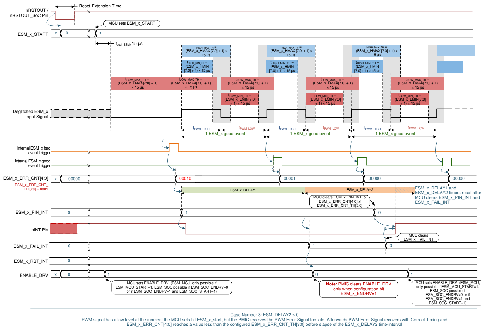
Figure 8-34. Example Waveform for ESM in PWM Mode – Case Number 3: ESM Starts with Low-Level at Deglitched Input Signal, but Receives Too Late a Correct PWM Signal Afterwards (The _x stand for _MCU or _SoC)
