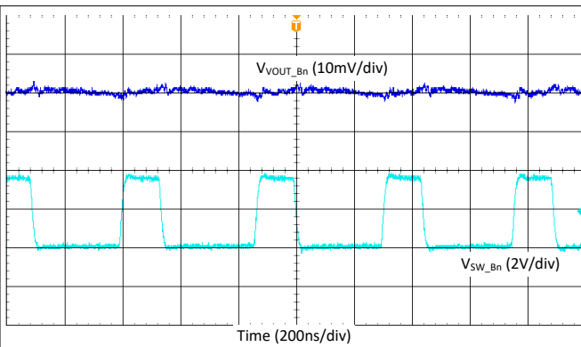
Figure 9-23. Buck Output Ripple - Single Phase, F_{sw} = 2.2\text{ MHz} , Forced-PWM Mode
