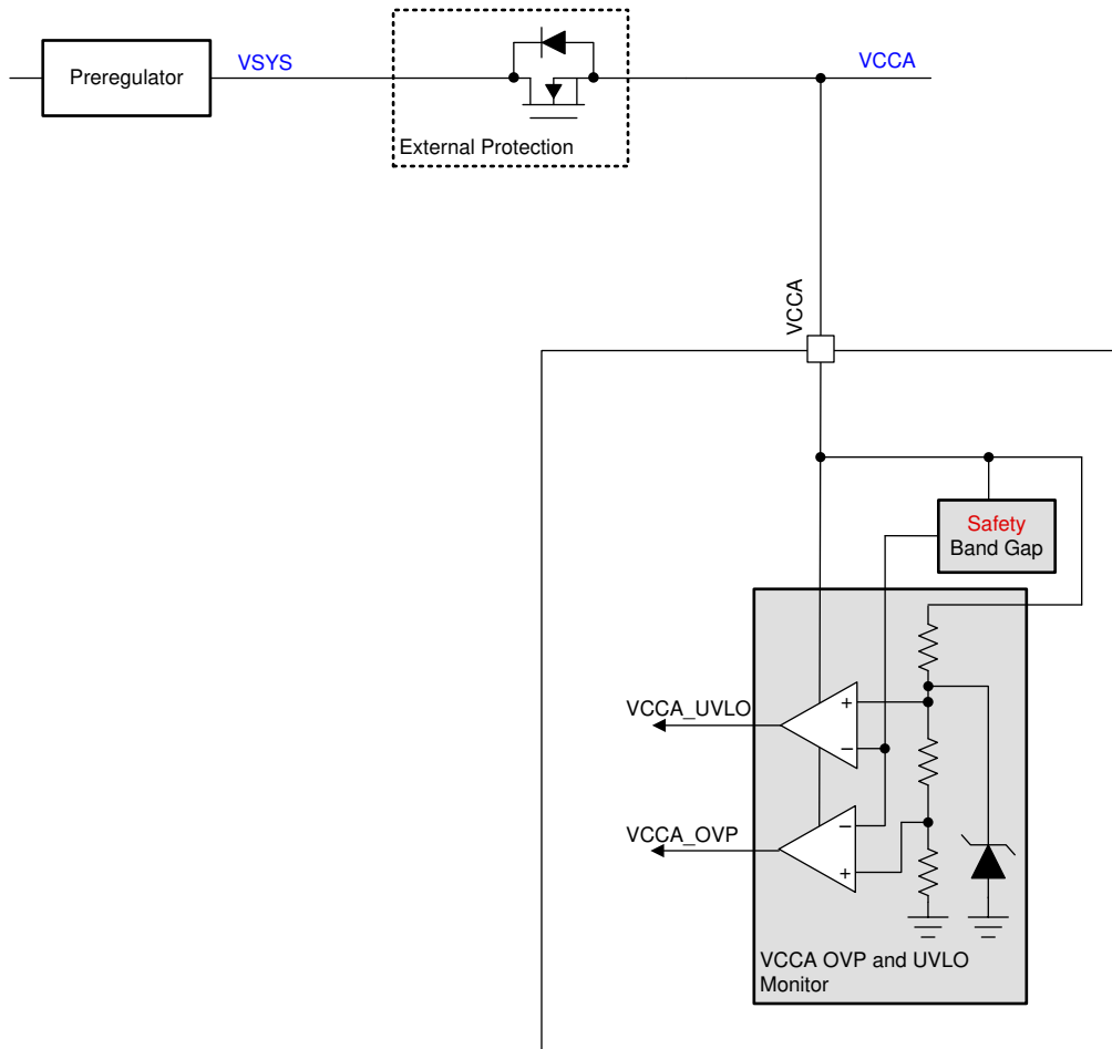
Figure 8-1. VCCA Monitor
