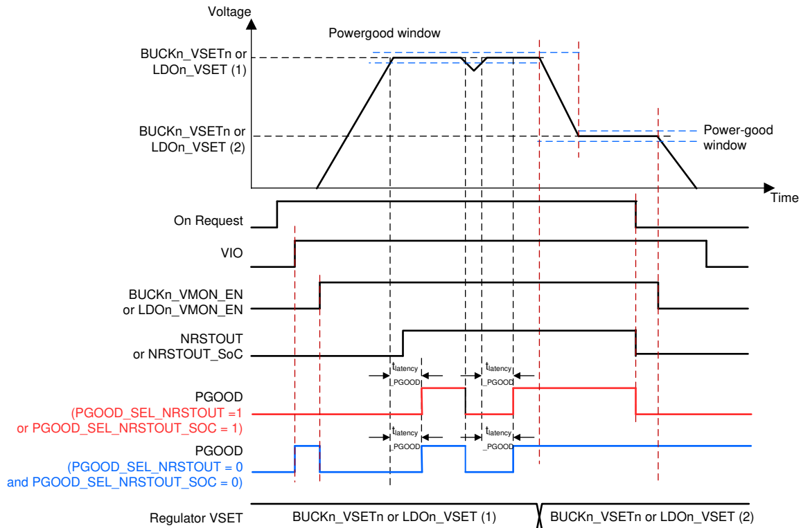
Figure 8-11. PGOOD Waveforms
