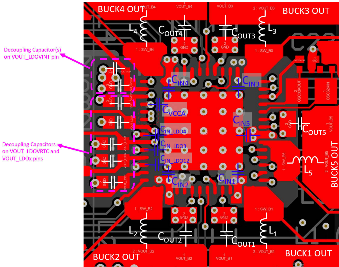
Figure 9-70. Example PMIC Layout
