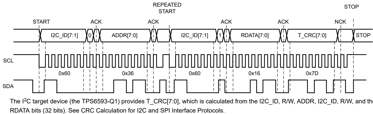
Figure 8-57. I 2 C READ Cycle with CRC
