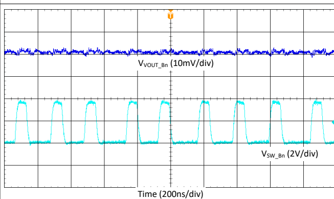
Figure 9-27. Buck Output Ripple - 2-Phase, F_{sw} = 4.4\text{ MHz} , Forced-PWM Mode
