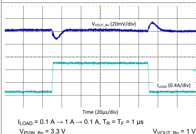
Figure 9-56. Buck Load Step Transient - Buck5, 2.2 MHz, Forced-PWM Mode
