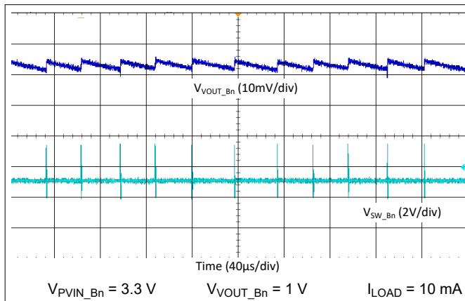
Figure 9-22. Buck Output Ripple - Single Phase, Auto Mode
