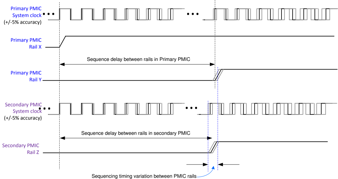
Figure 8-45. Multi-PMIC Rail Sequencing Timing Variation
