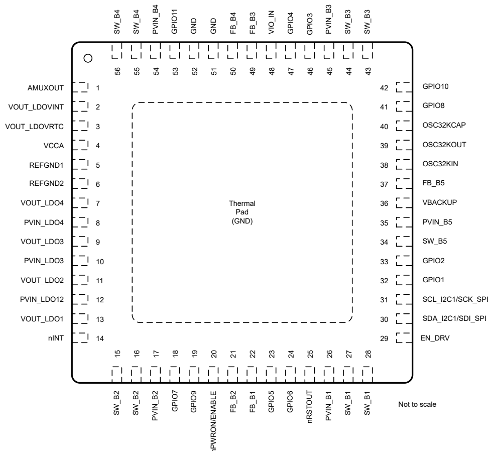
Figure 6-1. 56-Pin RWE (VQFNFP) Package, 0.5-mm Pitch, With Thermal Pad (Top View)
