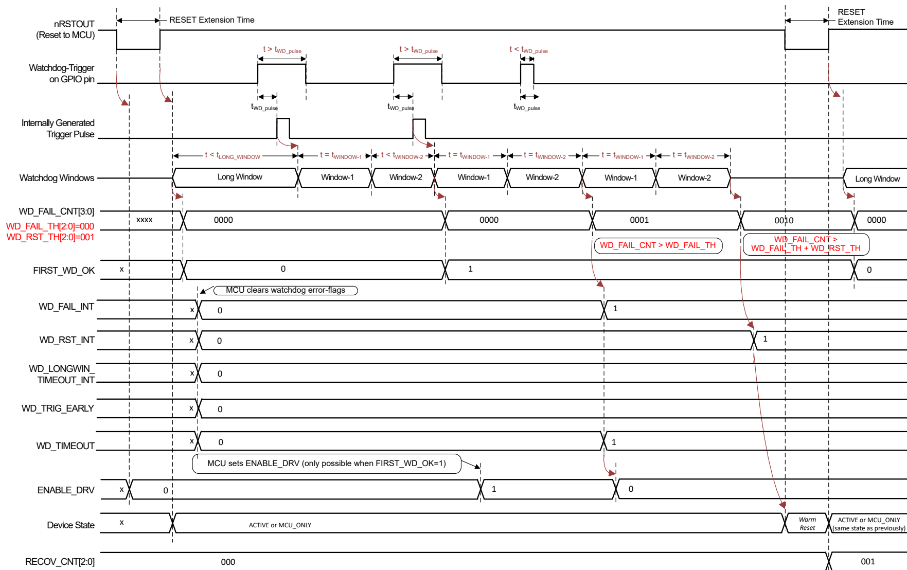
Figure 8-19. Watchdog in Trigger Mode – Bad Events (Too Short or no Trigger in Window-2) After Start-up
