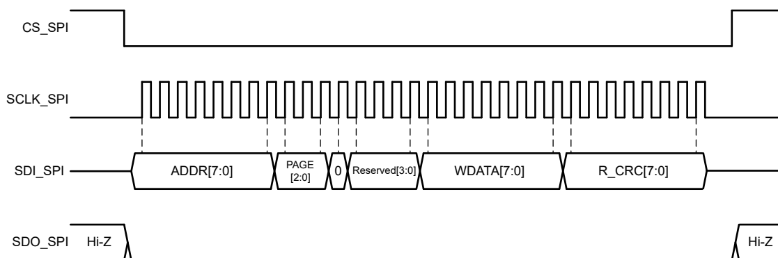
Figure 8-59. SPI Write Cycle with CRC
