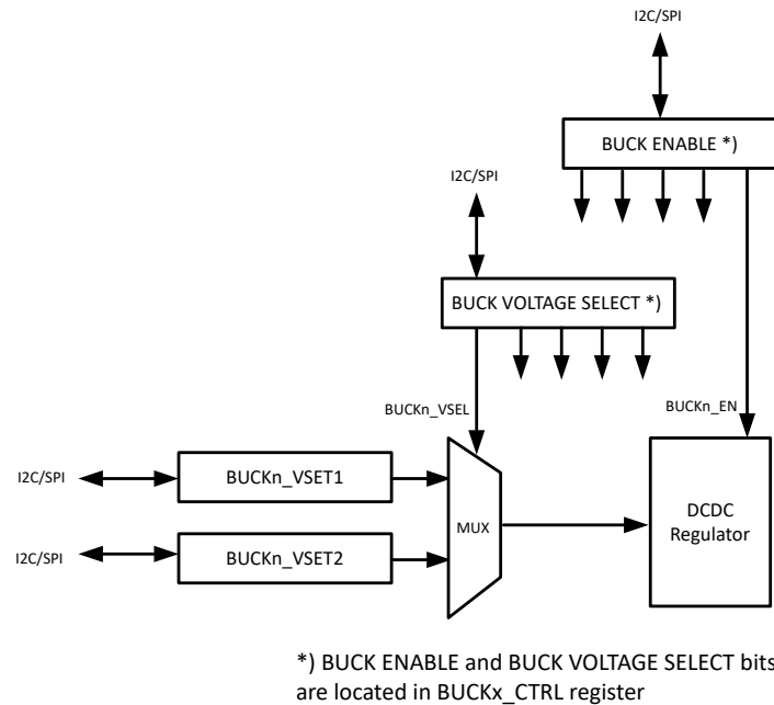
Figure 8-5. AVS/DVS Configuration Register Arbitration Diagram
