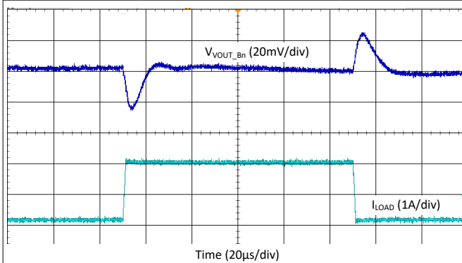
Figure 9-48. Buck Load Step Transient - 2-Phase, 2.2 MHz, Forced-PWM Mode
