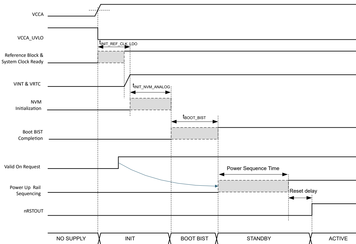
Figure 8-41. Device Start-up Timing Diagram
