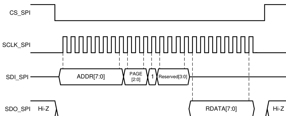
Figure 8-60. SPI Read Cycle
