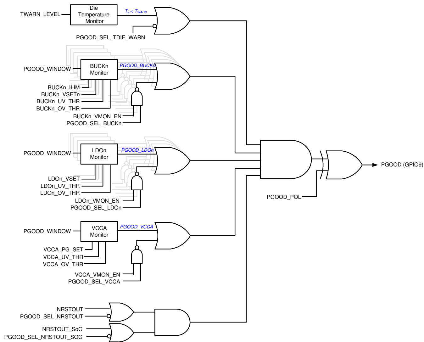
Figure 8-10. PGOOD Block Diagram
