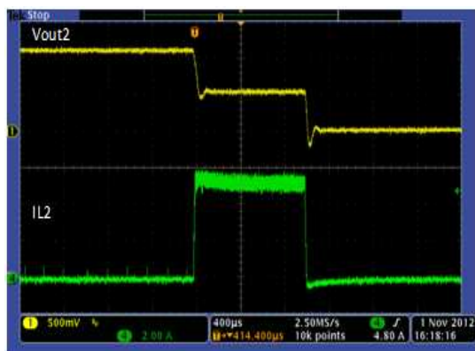
Figure 28. Over Current Protection, Buck 2
