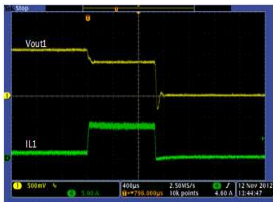
Figure 26. Over Current Protection Buck 1
