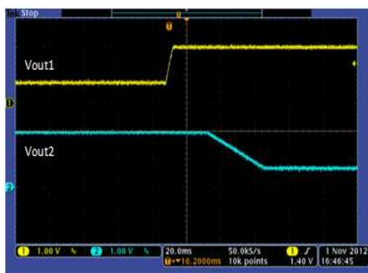
Figure 31. Voltage Change With I 2 C Control Buck 1, 0.68 V - 1.95 V, SR = 10\text{ mV}/16\text{ Tsw} , Buck 2, 1.95 V - 0.68 V, SR = 10\text{ mV}/128\text{ Tsw}
