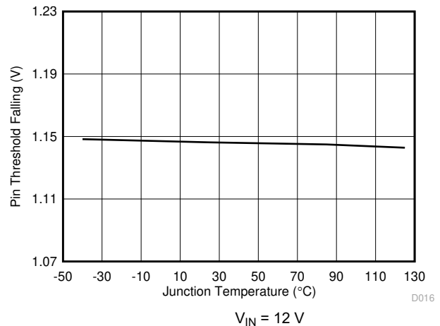
Figure 6-16. EN Pin Threshold Falling vs Temperature
