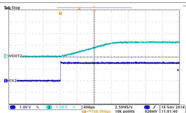
Figure 8-4. BUCK2, Soft Start
