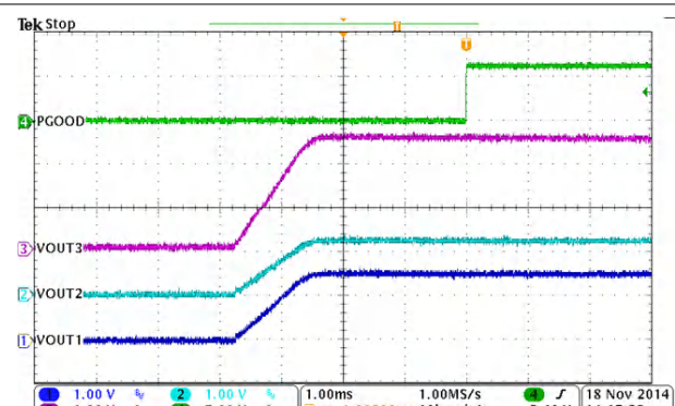
Figure 8-18. PGOOD
