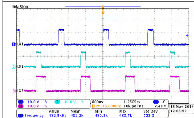
Figure 8-21. 180° Out-of-Phase
