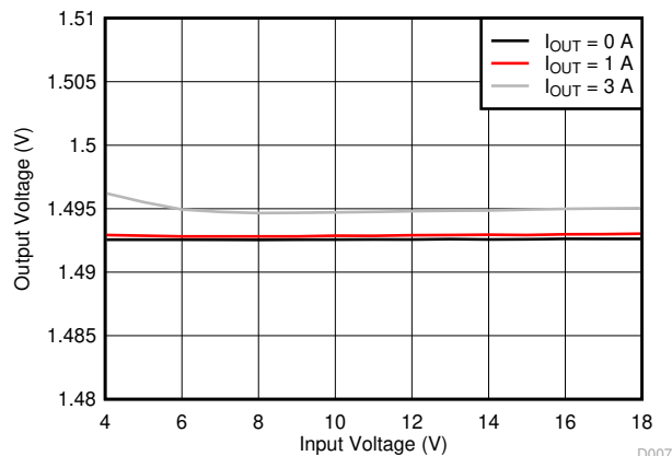
Figure 6-7. BUCK1, Line Regulation
