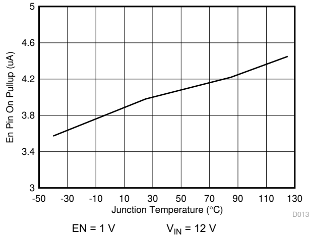
Figure 6-13. EN Pin Pullup Current vs Temperature, EN = 1.0 V
