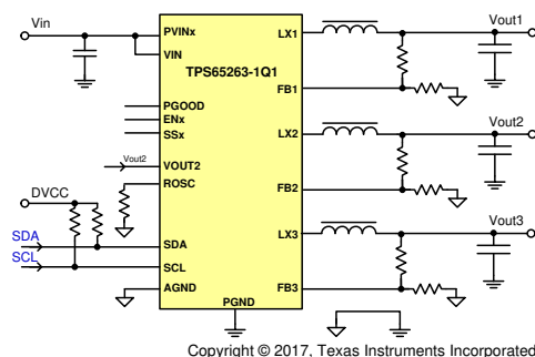
Application Schematic
