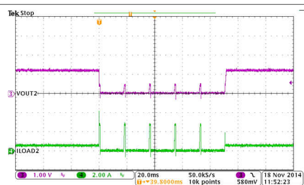
Figure 8-16. BUCK2, Hiccup and Recovery
