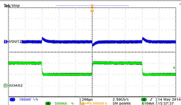
Figure 9-10. BUCK2, Load Transient, 0.5 to 1 A SR = 0.25 A/µs
