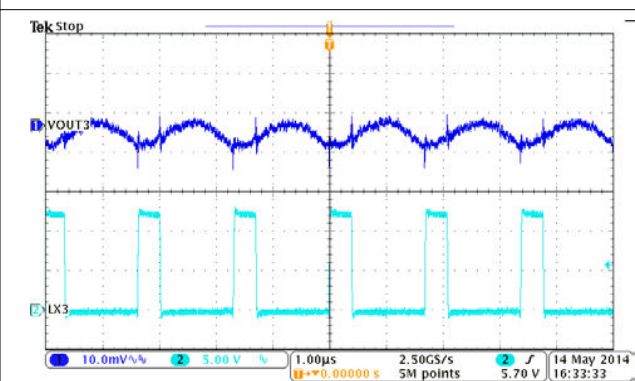
Figure 9-7. BUCK3, Output Voltage Ripple, Iout = 2 A
