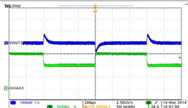
Figure 9-13. BUCK3, Load Transient, 1 to 1.5 A SR = 0.25 A/µs
