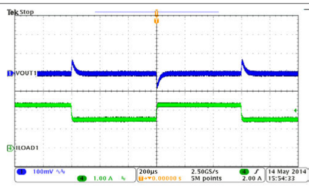
Figure 9-9. BUCK1, Load Transient, 1.5 to 2.25 A SR = 0.25 A/µs
