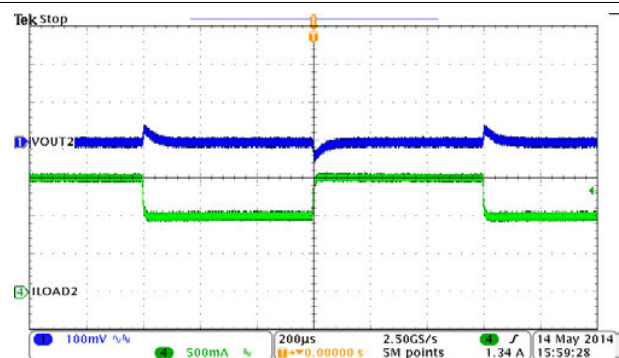
Figure 9-11. BUCK2, Load Transient, 1 to 1.5 A SR = 0.25 A/µs
