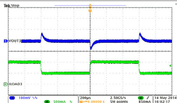
Figure 9-12. BUCK3, Load Transient, 0.5 to 1 A SR = 0.25 A/µs
