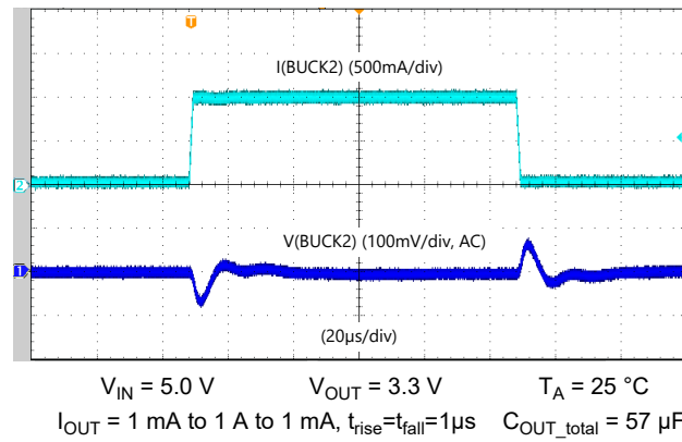
Figure 5-4. BUCK2 Load-step response - Low Bandwidth, forced PWM
