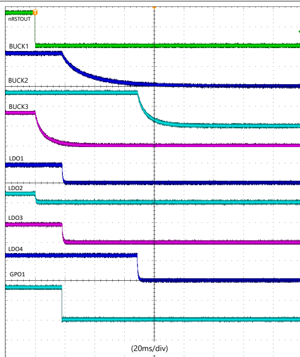
Figure 7-9. LDOs Discharge
