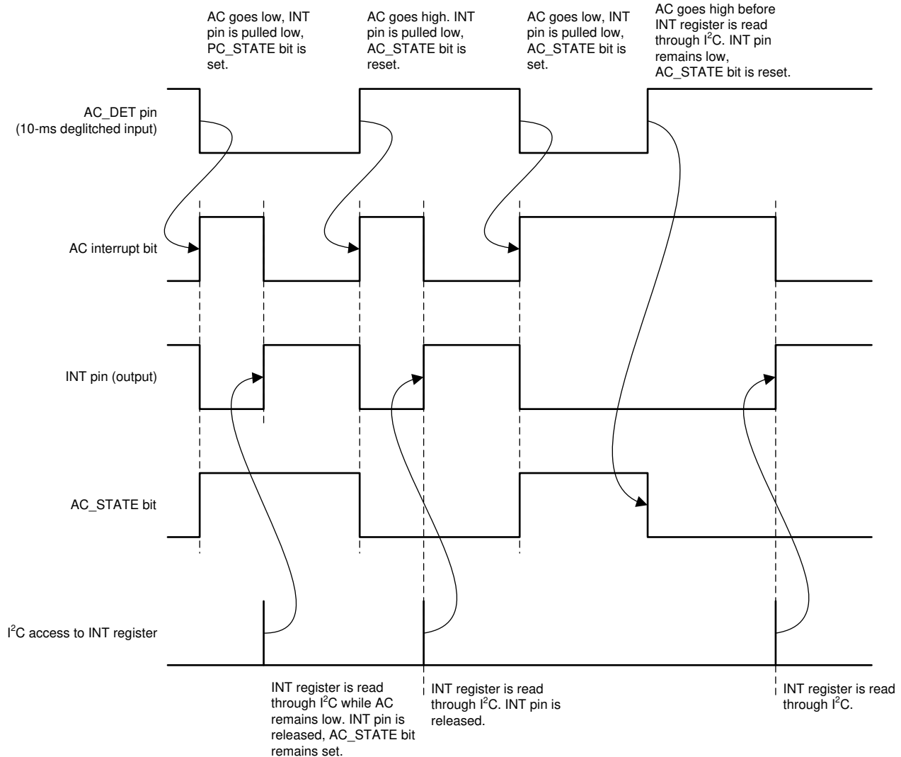
Figure 7-22. AC_STATE Pin
