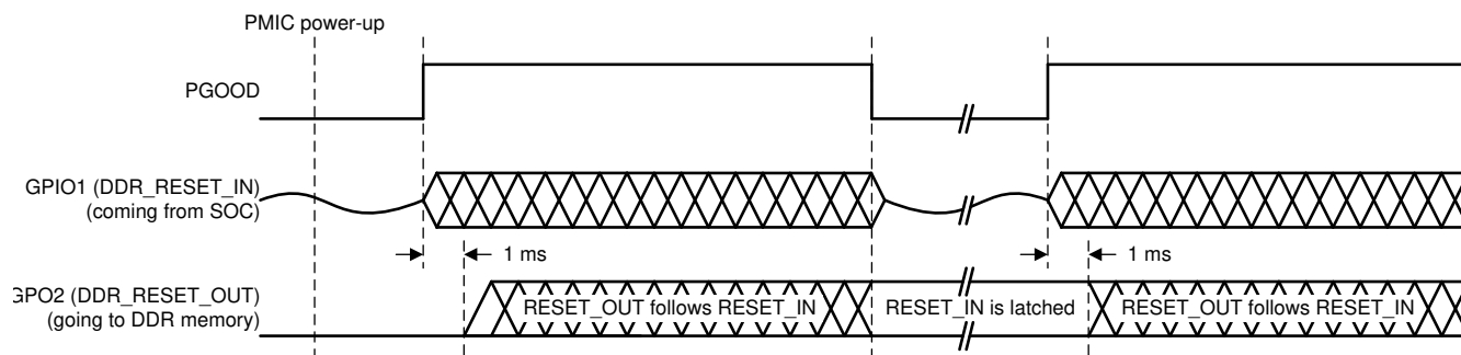
Figure 7-17. DDR3 Reset Timing Diagram
