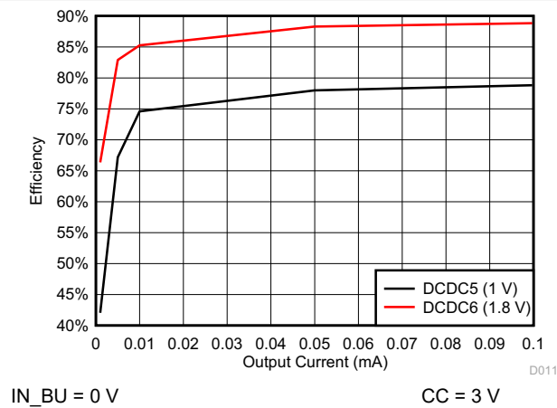
Figure 8-8. DCDC5/DCDC6 Efficiency
