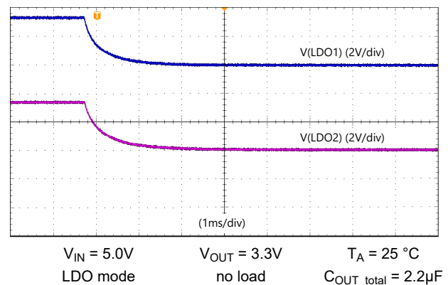
Figure 7-9. LDOs Discharge
