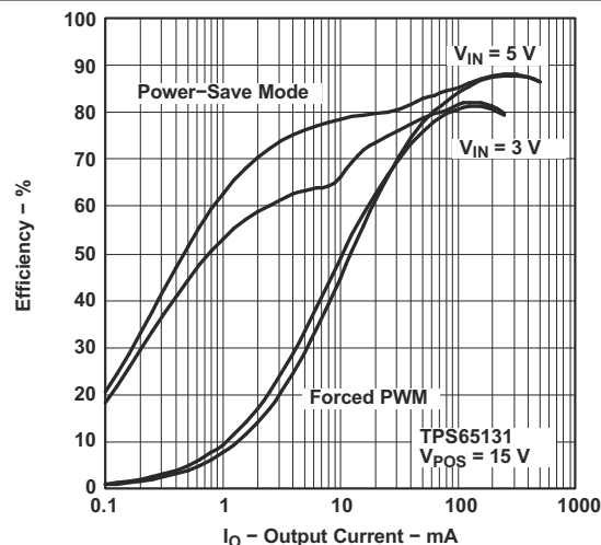
Figure 8-7. TPS65131 Efficiency vs Output Current
