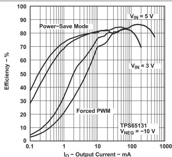
Figure 8-11. TPS65131 Efficiency vs Output Current
