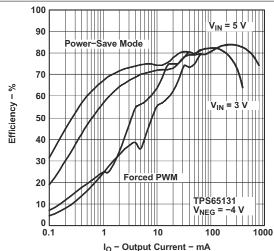
Figure 8-9. TPS65131 Efficiency vs Output Current
