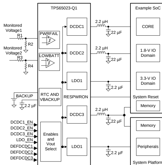
Simplified Schematic
